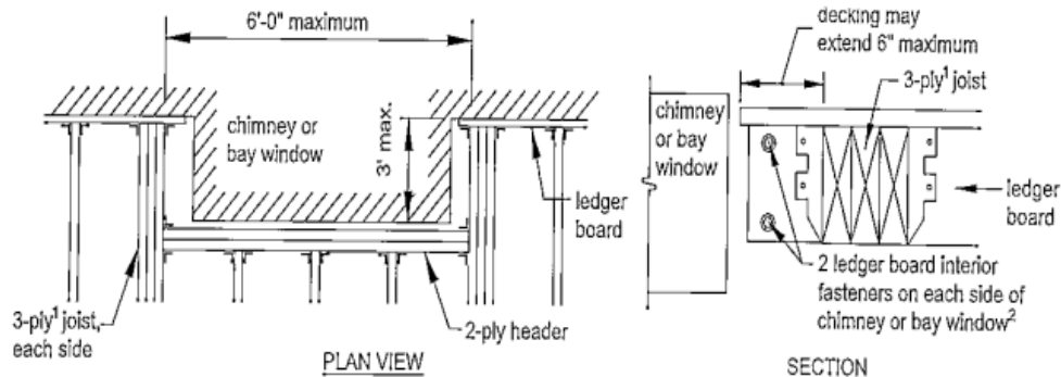
FIGURE 21: REQUIREMENTS FOR FRAMING AT CHIMNEY OR BAY WINDOW
