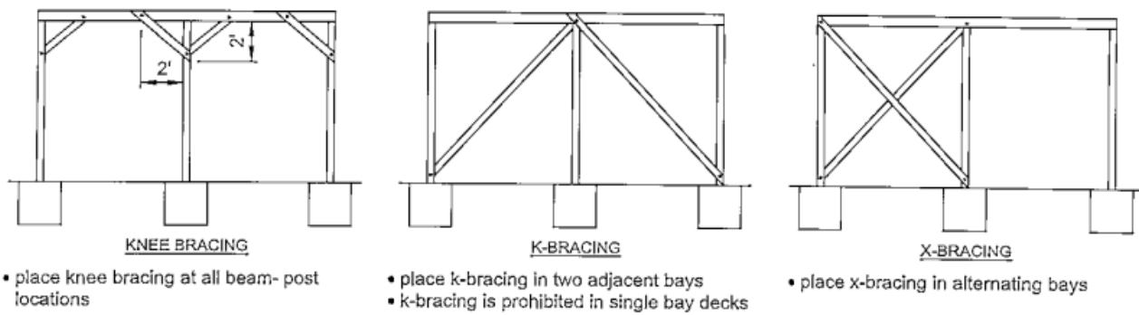
FIGURE 22: DIAGONAL BRACING AT BEAM-POST LOCATIONS (all decks)
