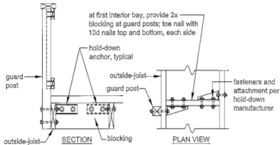
FIGURE 30: GUARD POST-TO-OUTSIDE JOIST DETAIL
