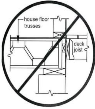
FIGURE 17: FLOOR TRUSSES
