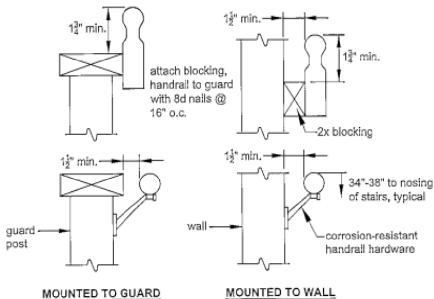
FIGURE 38: HANDRAIL REQUIREMENTS
