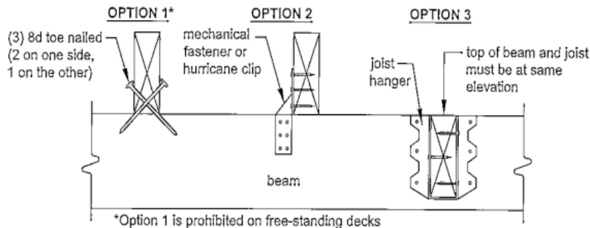
FIGURE 8: JOIST-TO-BEAM DETAIL
